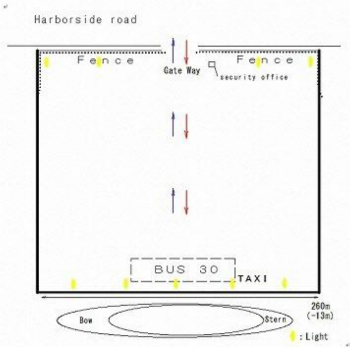
Figure of the terminal placement and passenger line of flow ターミナル配置図と受入動線
