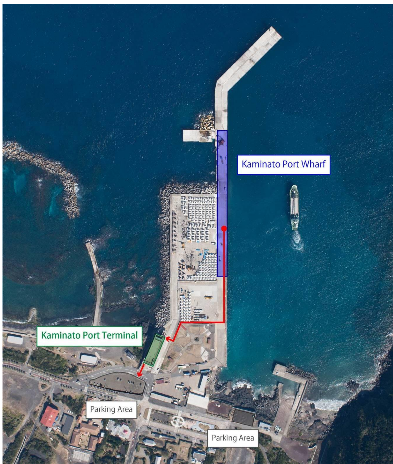
Figure of the terminal placement and passenger line of flow ターミナル配置図と受入動線
