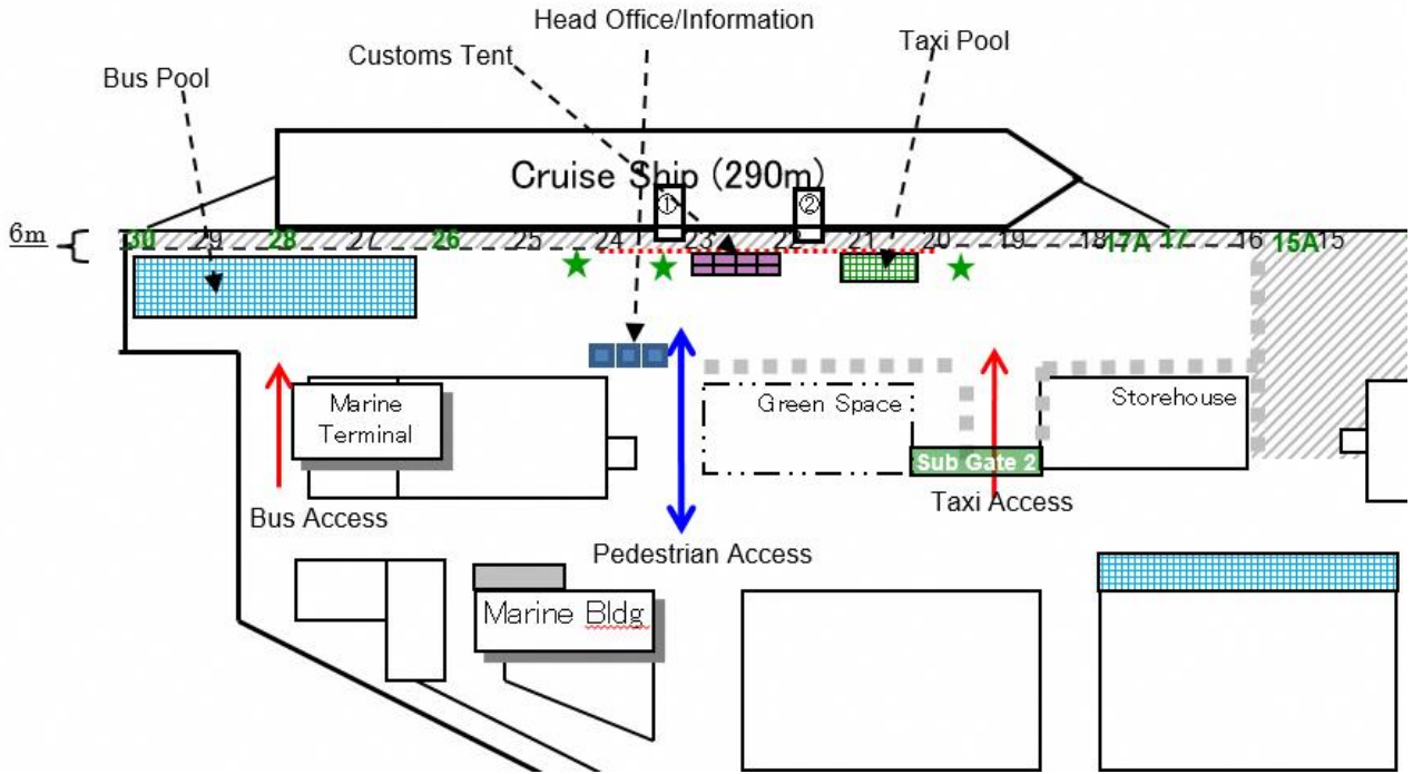
Figure of the terminal placement and passenger line of flow ターミナル配置図と受入動線
